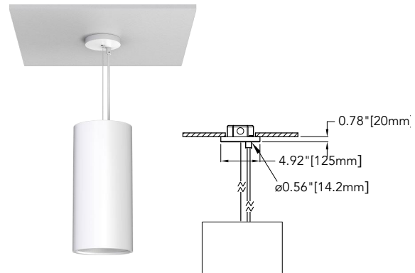
SCKG - Cable & lanyard canopy with recessed J-box (6" & 8")
